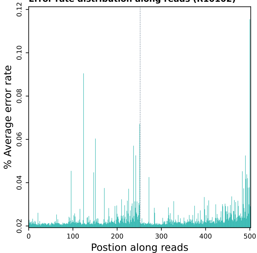
Error rate distribution along reads (R10102)
